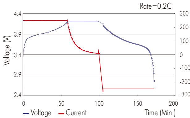
Charge & Discharge ( 23\pm 2^{\circ}\text{C} )
