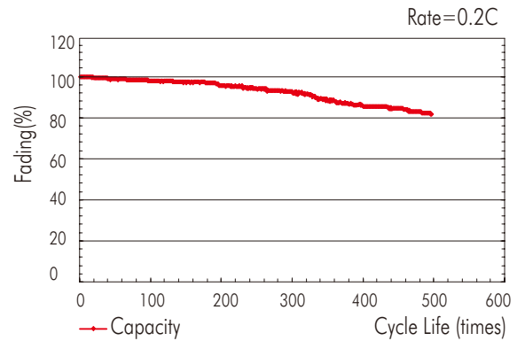
Cycle Life ( 23\pm 2^{\circ}\text{C} )
