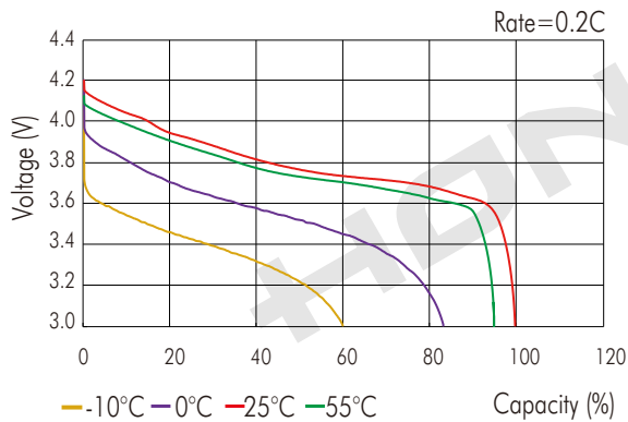
Discharge Characteristics (by Temp.)
