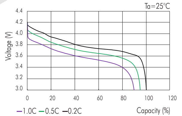
Discharge Characteristics (by rate)
