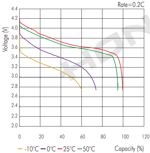
Discharge Characteristics (by Temp.)
