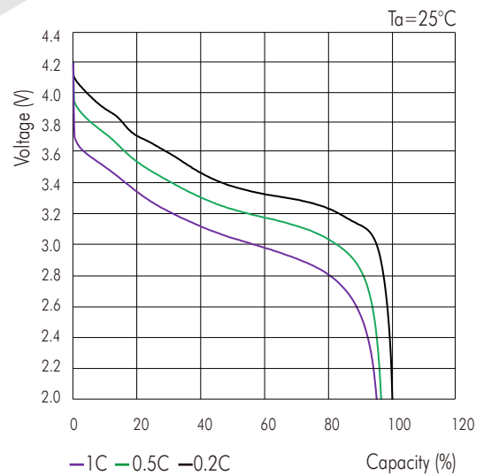
Discharge Characteristics (by rate)
