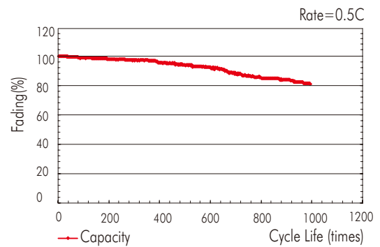
Cycle Life ( 23 \pm 2^\circ\text{C} )
