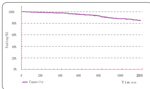
Cycle Life
