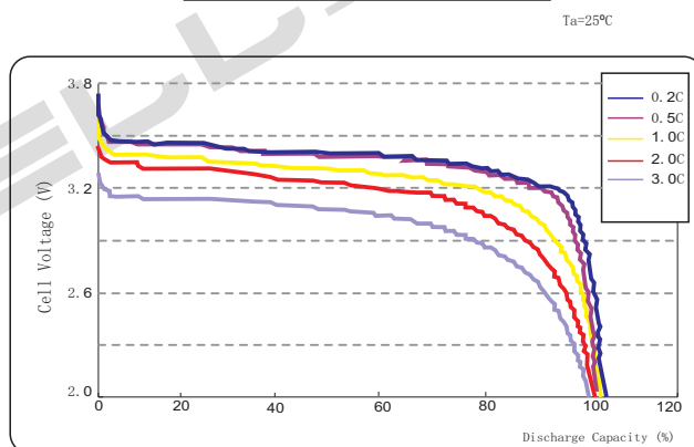
Discharge Characteristics (Rate)
