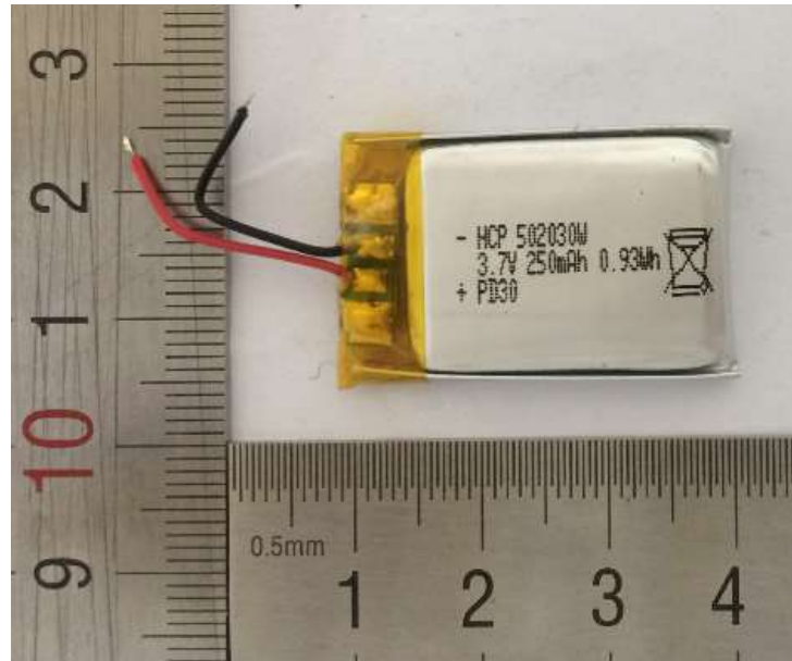
Figure 1 Front view of battery
