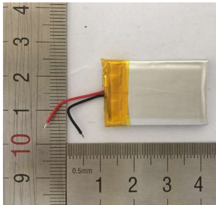
Figure 2 Back view of battery
