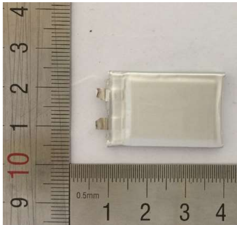
Figure 6 Back view of cell
