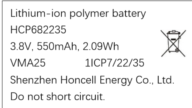
Battery Label
