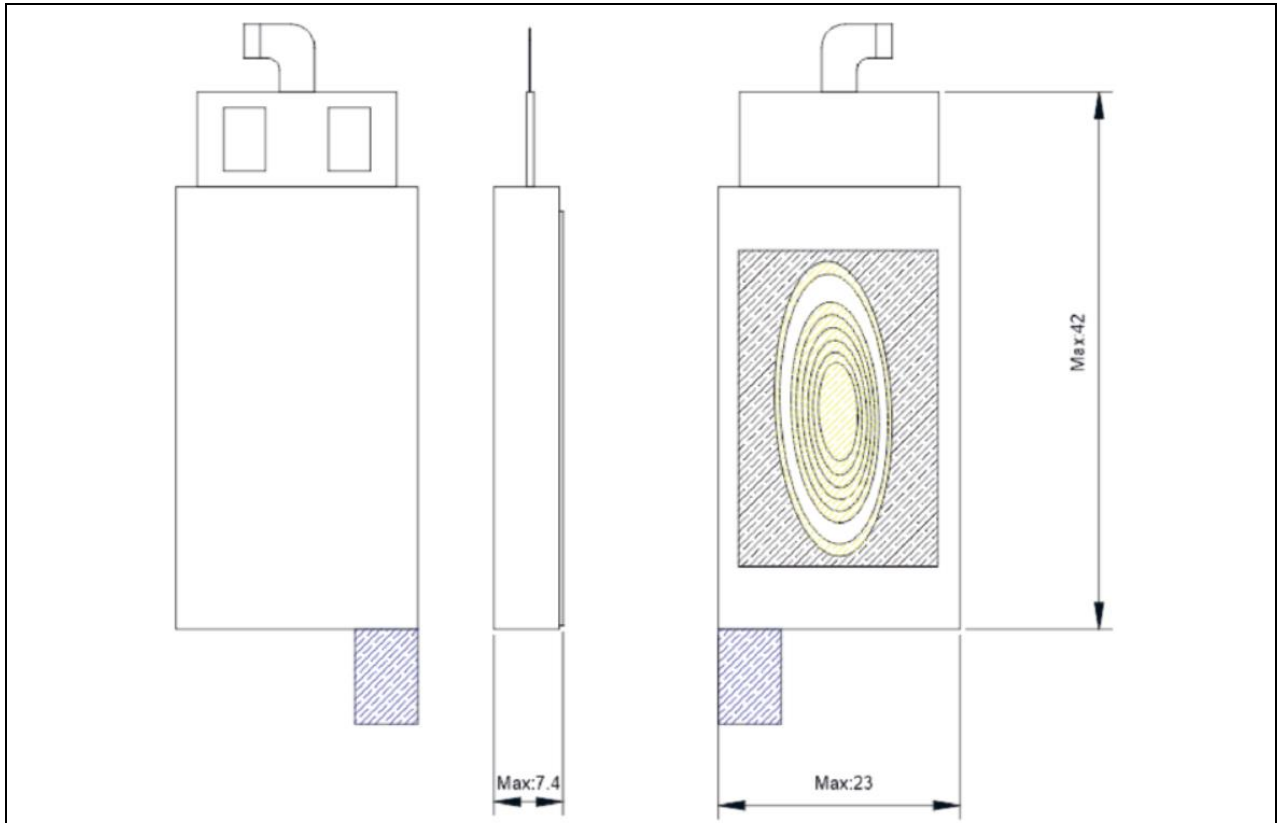
Battery (Unit: mm)
