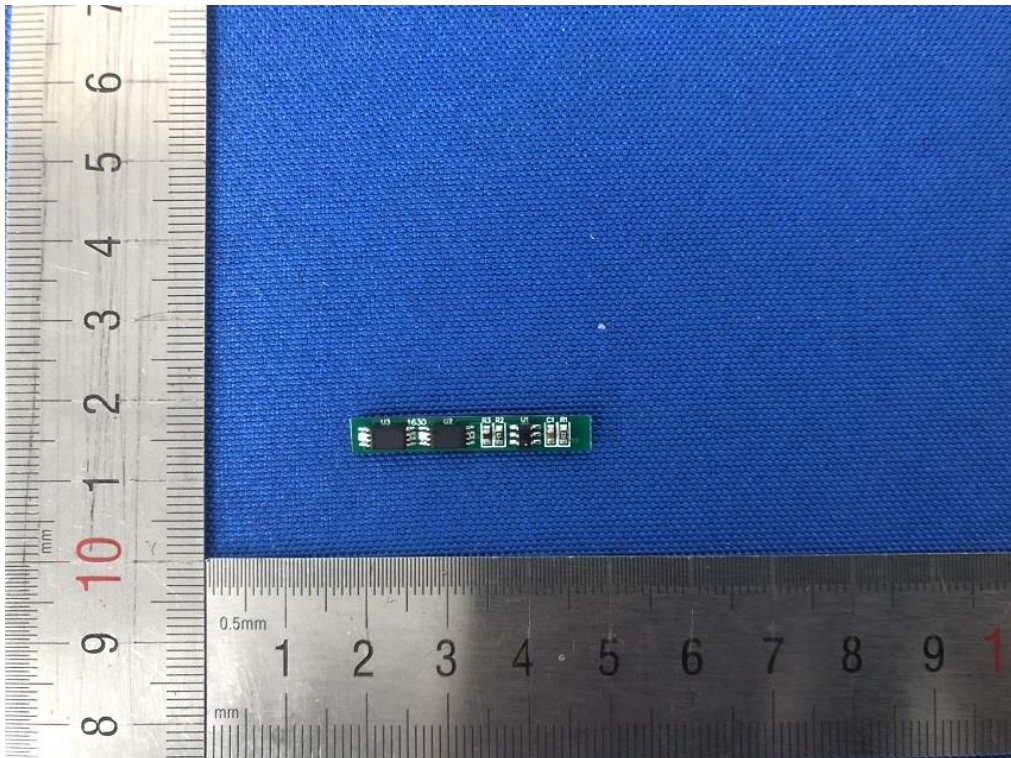
Figure 6 Front view of PCB
