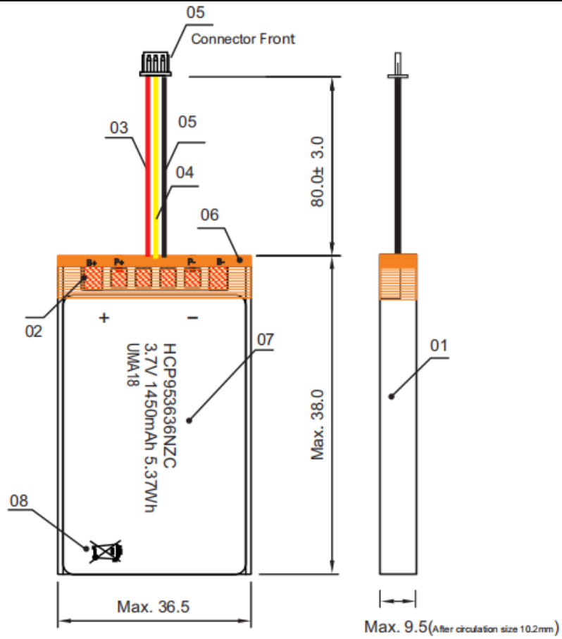
Battery (Unit: mm)
