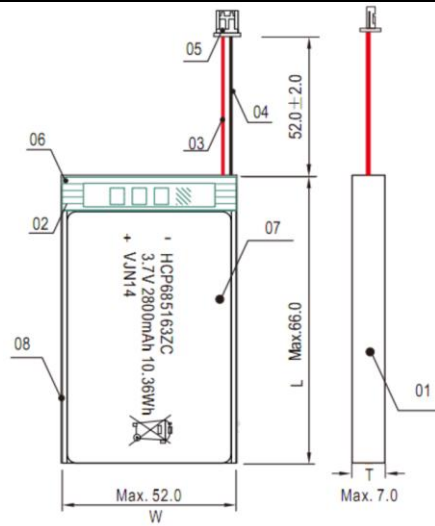
Battery (Unit: mm)
