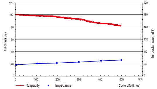
Cycle Life
